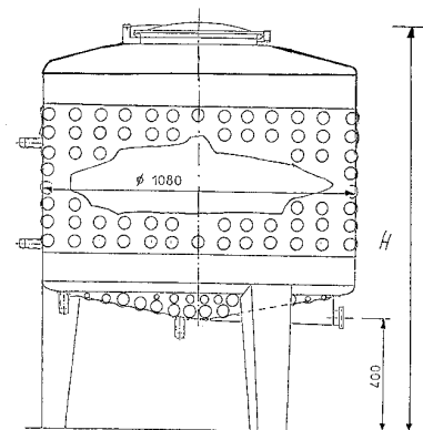
Version 2 Mannloch Ø 400 mm
